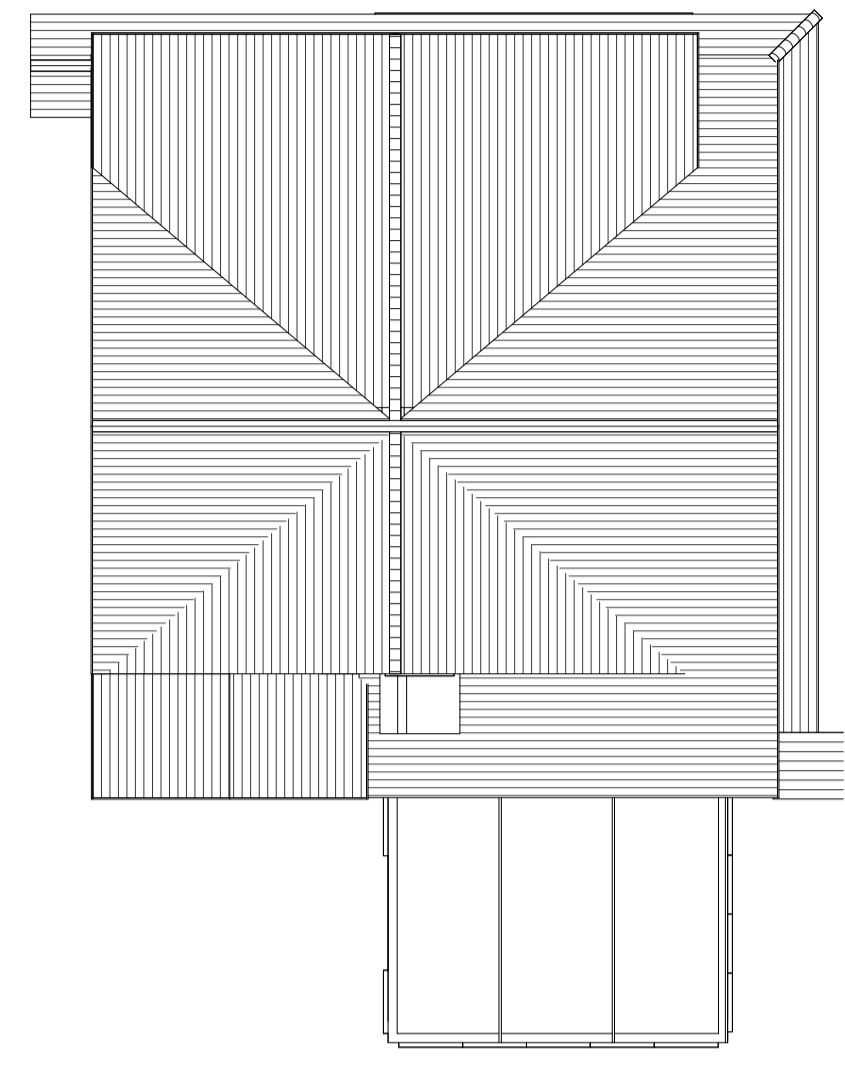
Previous Existing Roof Plan 1 : 100
