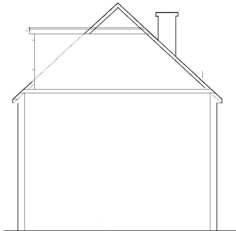
PROPOSED SECTION
