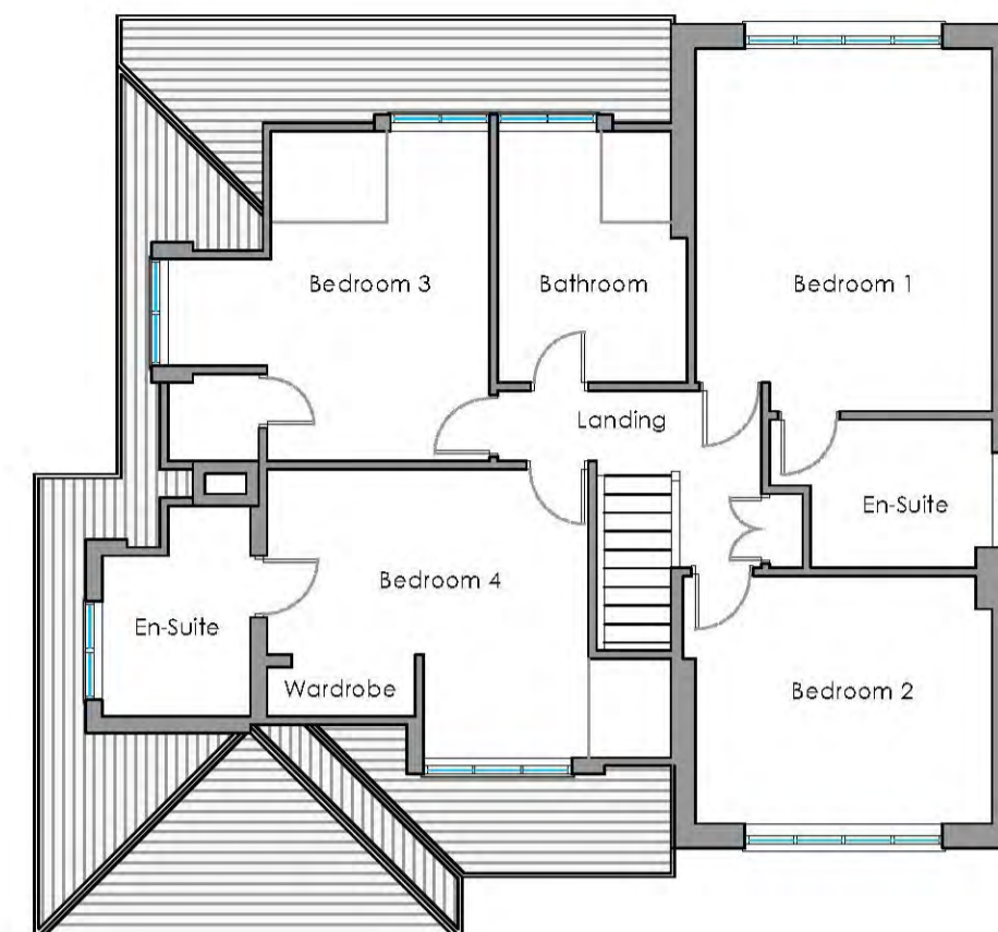
2 Existing First Floor Plan Scale: 1:100
