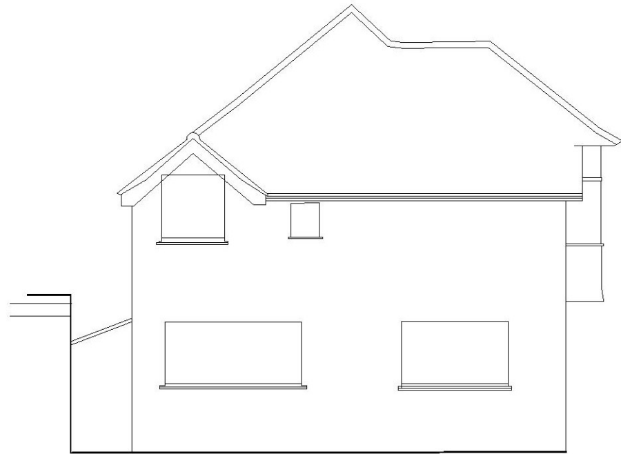
NORTH ELEVATION
