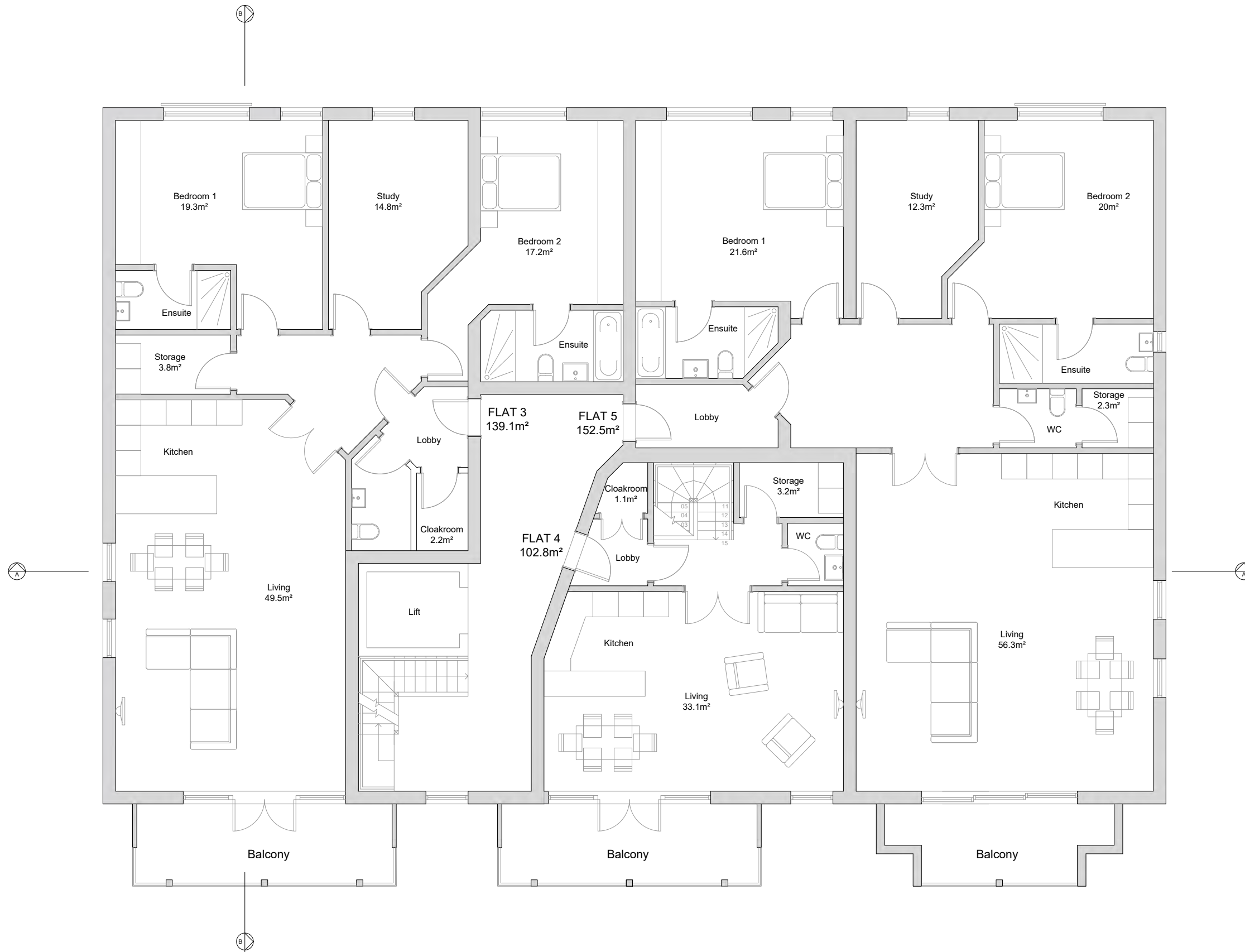
PROPOSED 1ST LEVEL PLAN 1:100
