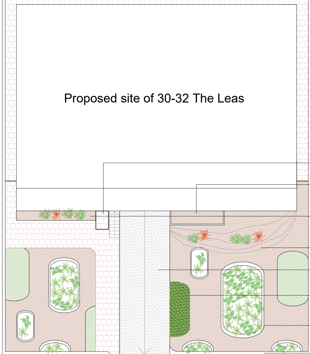
PROPOSED LANSCAPE PLAN 1:200 @ A3
