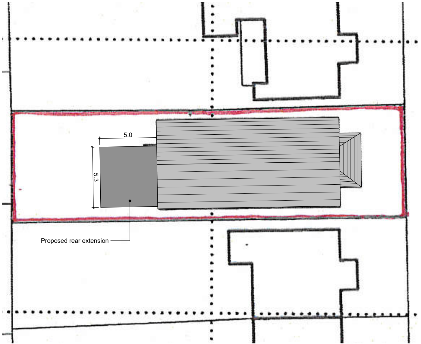
Block Plan
