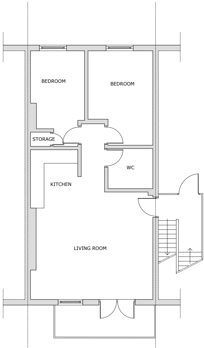
EXISTING SECOND FLOOR PLAN SCALE 1:100
