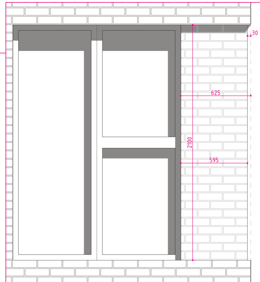
1:20 DETAIL
