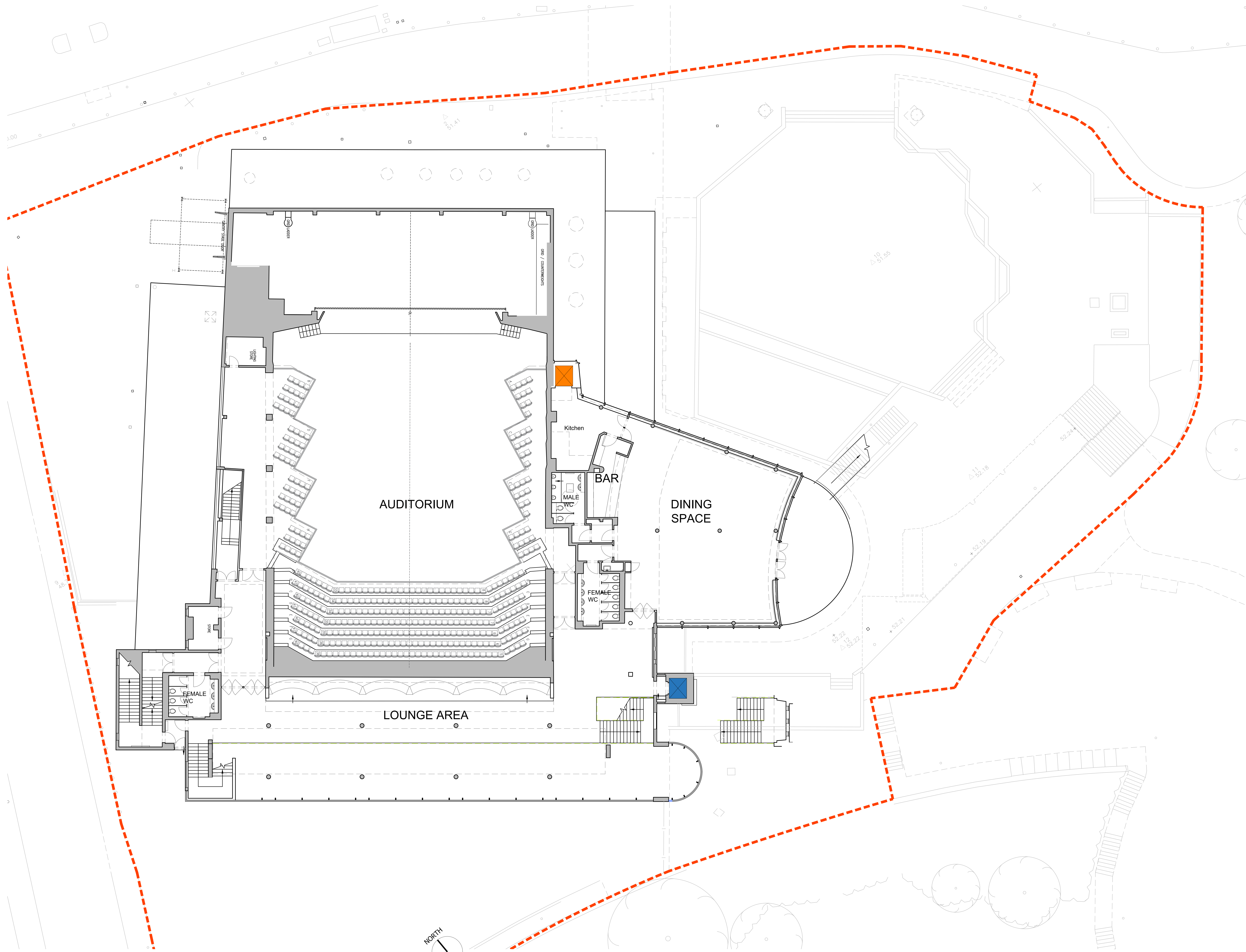
1 EXISTING FIRST FLOOR GA PLAN 1:100@A0
