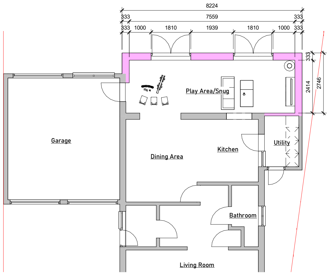
01 - Ground Floor 1 : 100
