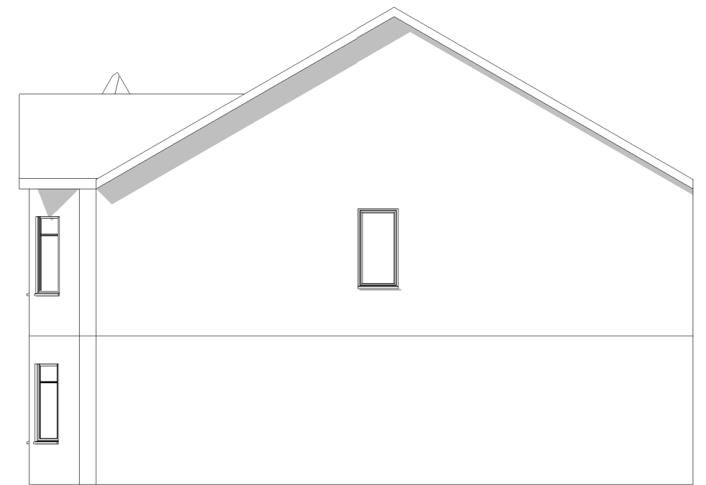
Existing Left Side Elevation 1 : 100
