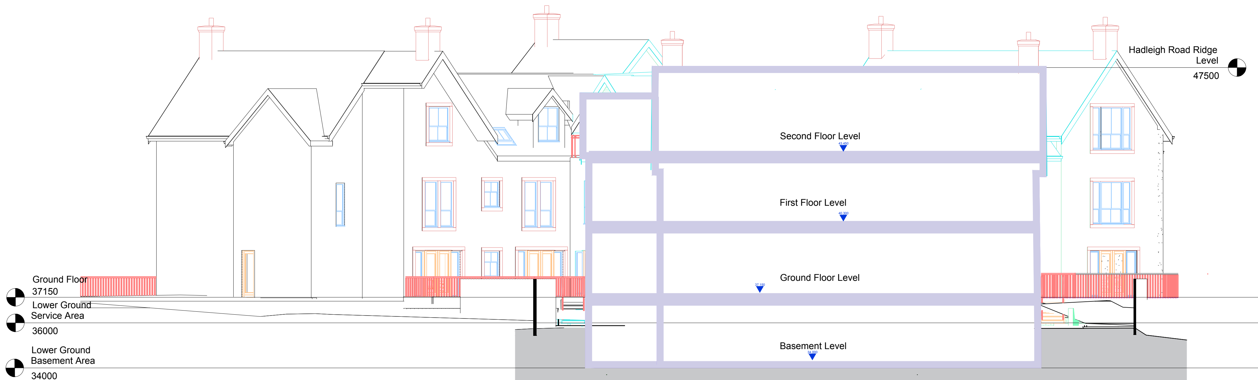
Proposed Basement Section A-A 1:100
